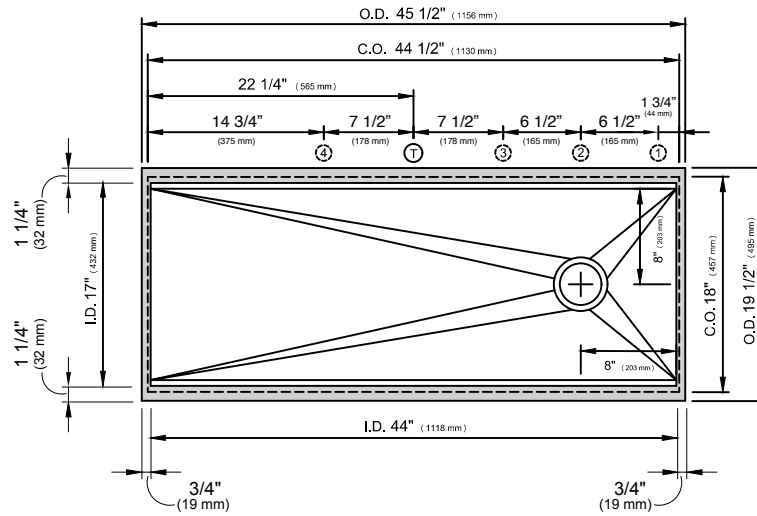
COUNTERTOP CUTOUT PLAN
